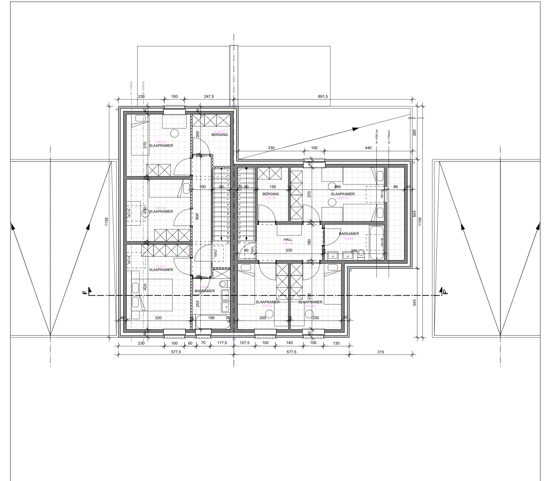
Typechakeling CD + carports - VERDIEPING 1
