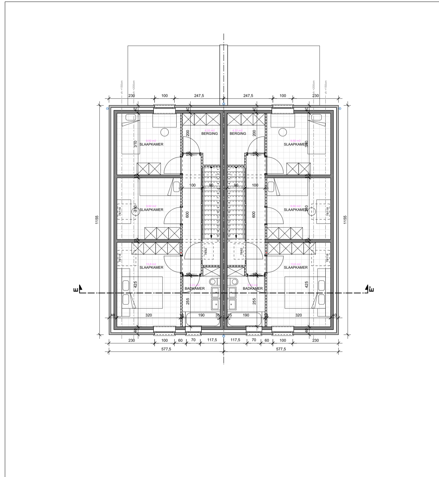
Typechakeling CC - VERDIEPING 1
